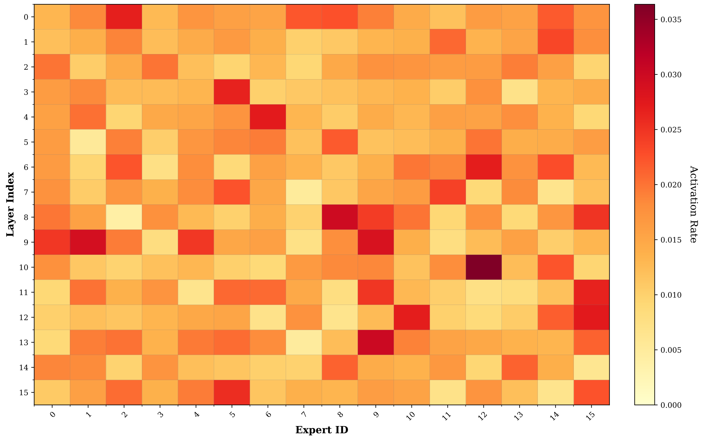
Expert Activation Patterns - deepseek-moe-16b-base_real_e64
